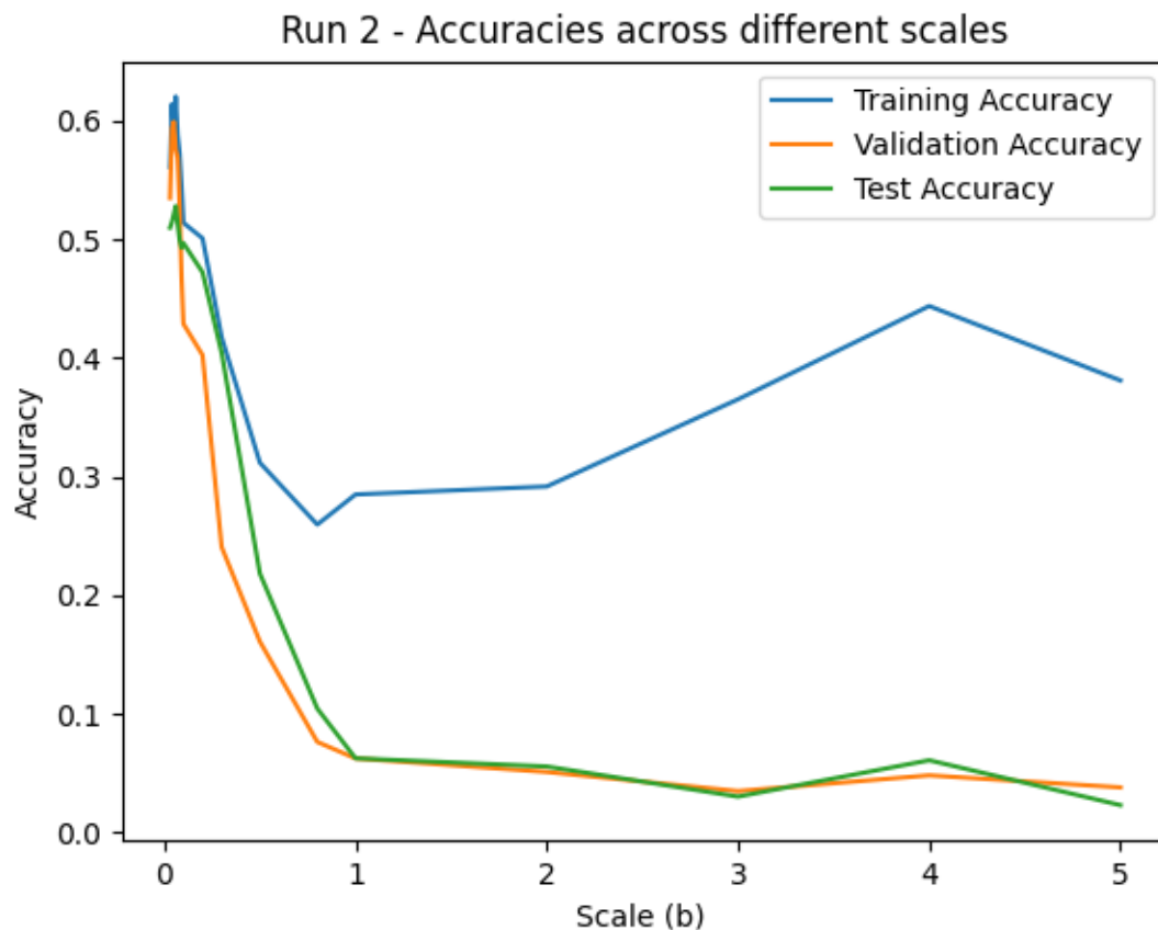
Figure 9: The curves showing the accuracy values across different noise scale values
