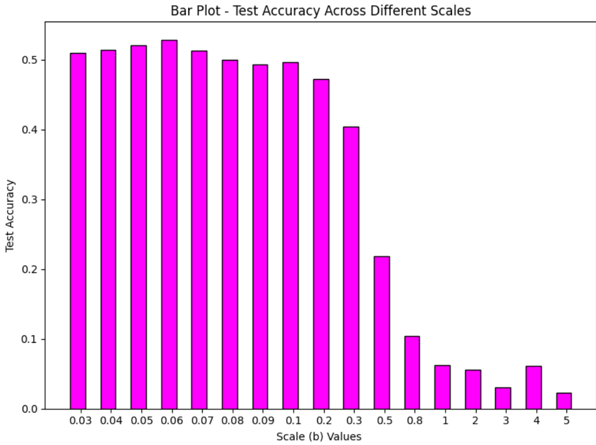
Figure 10: Bar Plot of the Test Accuracy across different scale values
